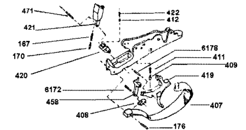
SELECTIVE TRIGGER GROUP
