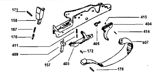
ADJUSTABLE TRIGGER GROUP
