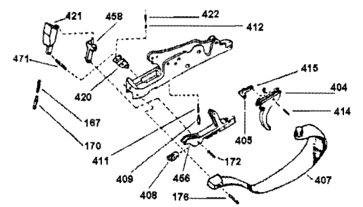
ADJUSTABLE AND SELECTIVE TRIGGER GROUP
