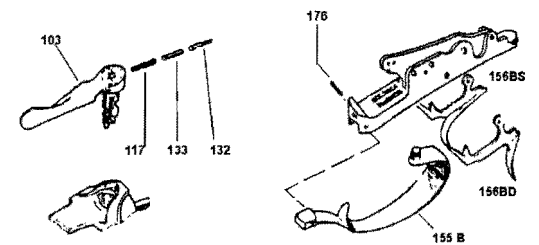
OLD TYPE TOP LEVEL ASSEMBLY
