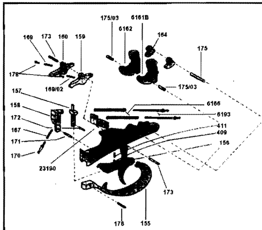
COMPONENTS FOR DETACHABLE TRIGGER GROUP WITH COIL SPRINGS
